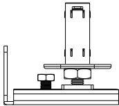
Wall/ Floor Fix Bottom Pivot
